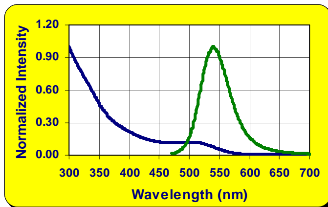
Absorption and emission spectra of ADS540QD quantum dot in aqueous solution.
