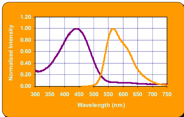
Absorption and emission spectra of ADS504PT in THF solution
