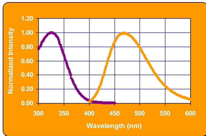
Absorption and emission spectra of ADS410PT in THF solution
