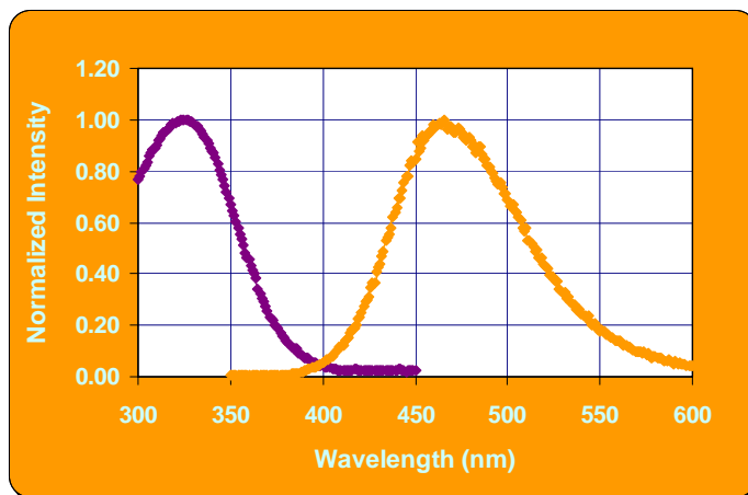
Absorption and emission spectra of ADS404PT in THF solution
