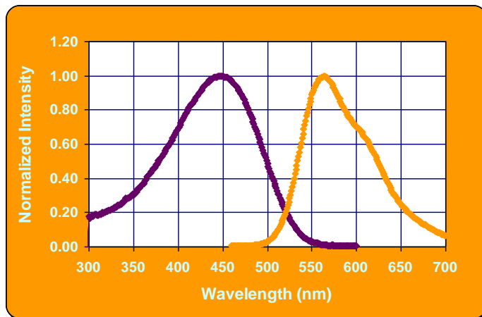
Absorption and emission spectra of ADS310PT in THF solution
