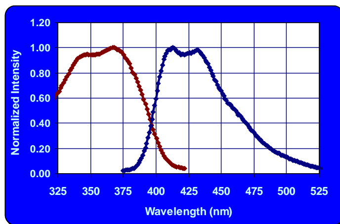
Absorption and emission spectra of ADS136FS in THF solution.
