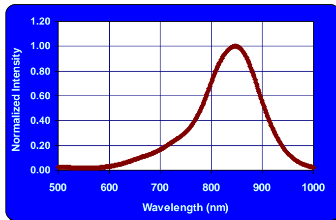
Absorption spectrum of ADS845MC in acetone
