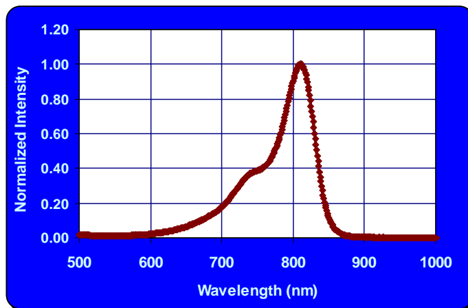
Absorption spectrum of ADS800AT in methanol
