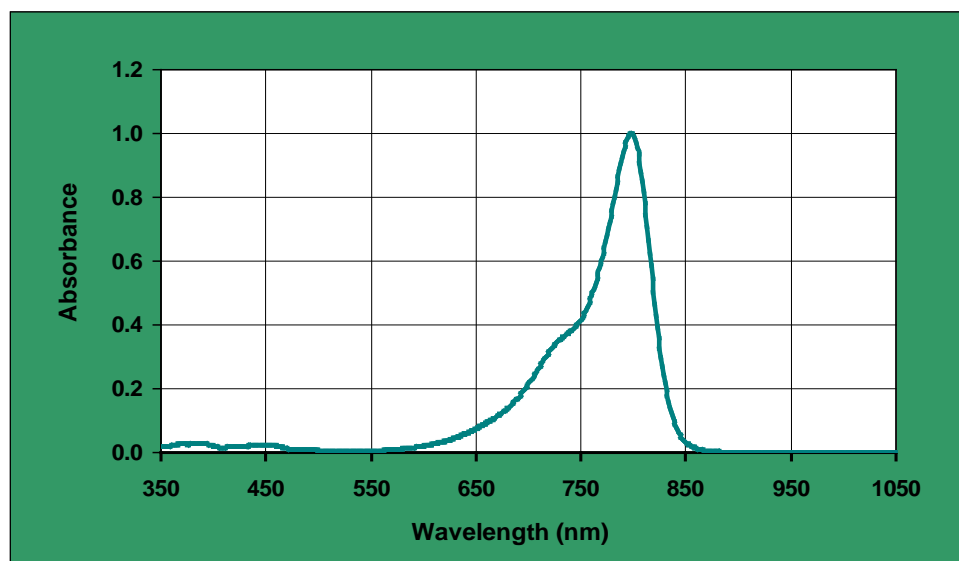
Absorption spectrum of ADS798SM in methanol
