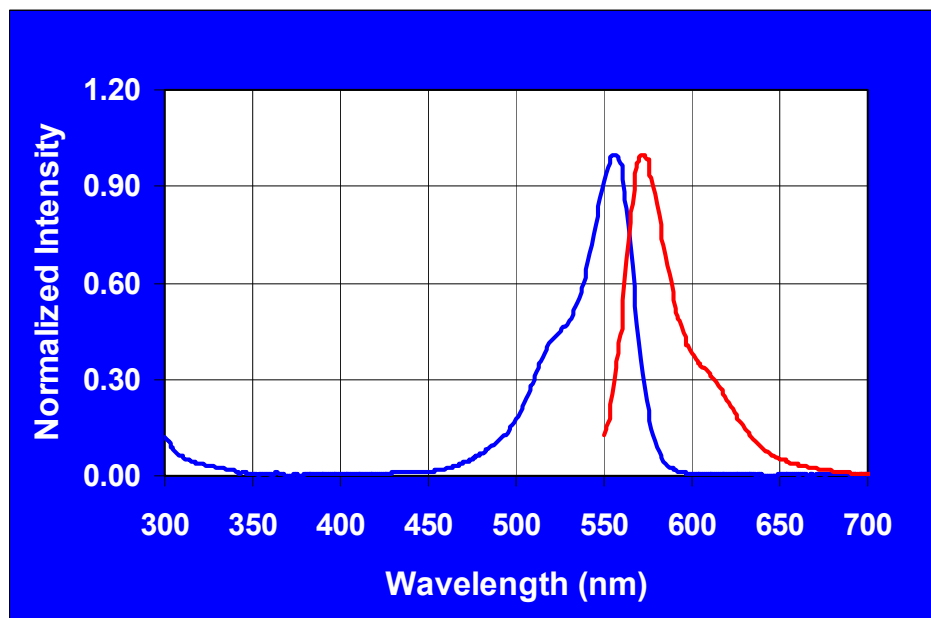
Absorption and Fluorescent Spectra of ADS560EI in methanol
