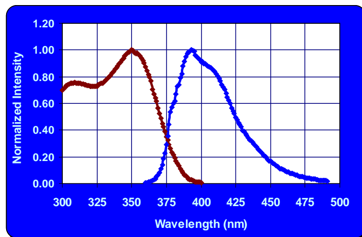
Absorption and photoluminescent spectra of ADS01HTM in THF solution
