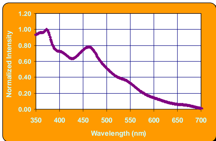
Absorption spectra of ADS71BFA in toluene solution
