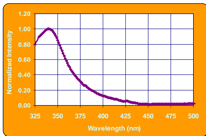
Absorption spectra of ADS65BFA in toluene solution
