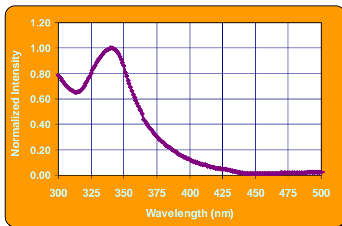
Absorption spectra of ADS64BFA in toluene solution
