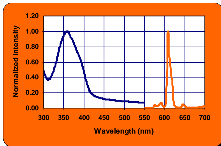
Absorption and photoluminescent spectra of ADS051RE in THF solution
