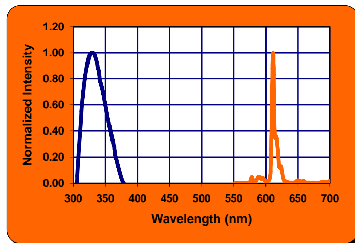
Absorption and photoluminescent spectra of ADS050RE in THF solution
