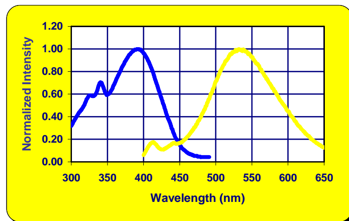
Absorption and photoluminescent spectra of ADS046YE in THF solution
