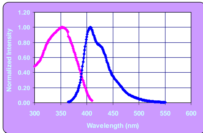
Absorption and emission spectra of ADS145UV In THF.
